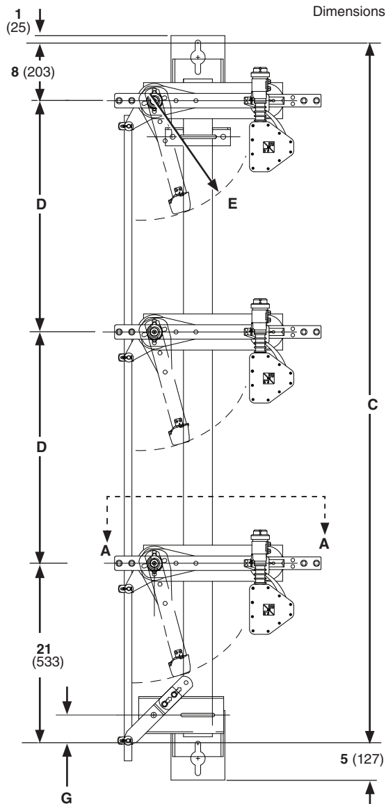
RECIPROCATING OPERATING MECHANISM
