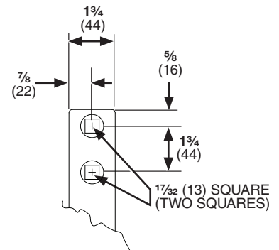
TERMINAL PAD DETAIL
