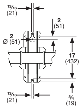
STANDARD MOUNTING BRACKET DETAIL
